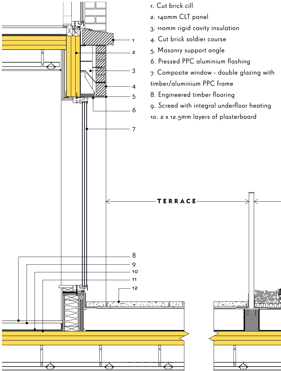
Plano. Waugh Thistleton.
